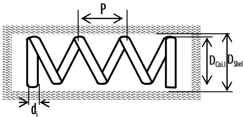
Fig. 3 Coiled tube heat exchanger
