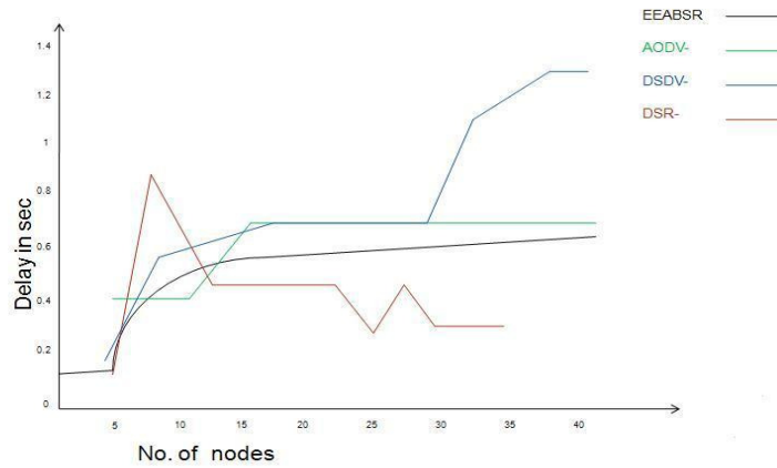
Figure 27: Graphical comparison of EEABSR with existing protocols
