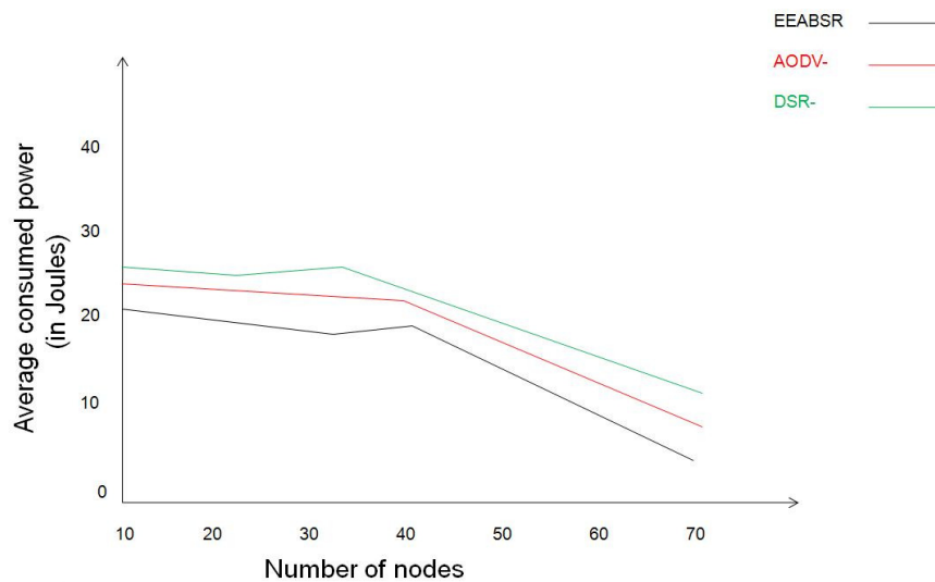
Figure 29: Average consumed power by EEABSR, AODV & DSR
