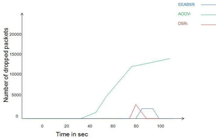
Figure 28: Packets Dropped by EEABSR, AODV & DSR
