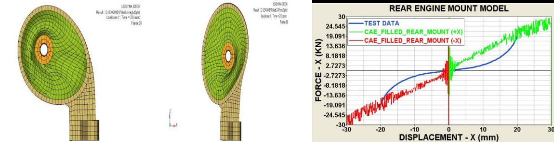
Fig.10 (a): Displacement of model in X-directions at 20 ms Fig.10 (b): Force Vs Displacement curve in Positive and Negative X directions
