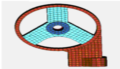
3(e) Design of Filler Arm Engine Mount
