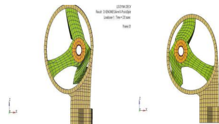
(b) Design of Three Arm Engine Mount
