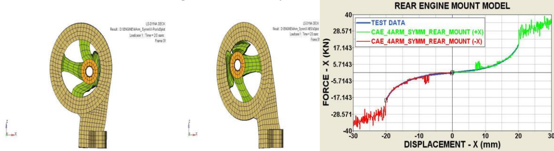
Fig.12 (a): Displacement of model in X-directions at 20 ms Fig.12 (b): Force Vs Displacement curve in Positive and Negative X directions
