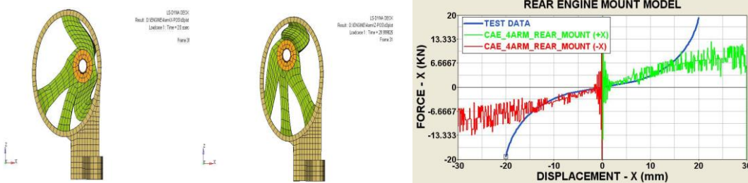
Fig.8 (a): Displacement of model in X-directions at 20 ms Fig.8 (b): Force Vs Displacement curve in Positive and Negative X directions
